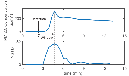
Figure 4: The illustration of the principle of the pollution event detection algorithm. The upper plot shows the PM 2.5 sensor data of the pesticide spray pollution event. The lower plot shows the corresponding NSTD values.
