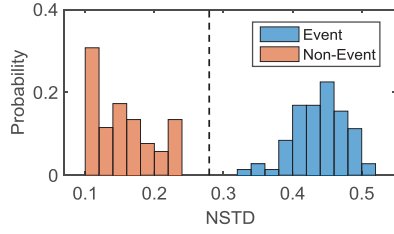
Figure 5: The normalized histogram of maximum NSTD values of pollution events vs. non-pollution events.
