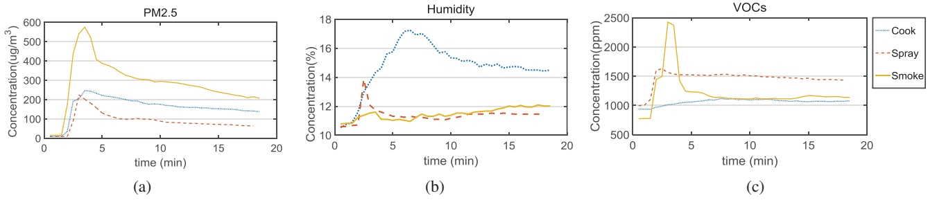
Figure 1: The (a) PM 2.5, (b) humidity, and (c) VOCs sensor measurements of indoor air pollution generated by cooking, smoking, and spraying pesticide.
