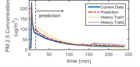
Figure 7: The illustration of the IAQ forecast algorithm in the context of predicting the PM 2.5 sensor values of a trial of pesticide spray.
