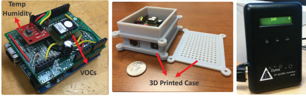
Figure 3: The IAQ sensing platform (left), the 3D printed case (middle), and the PM sensor (right).
