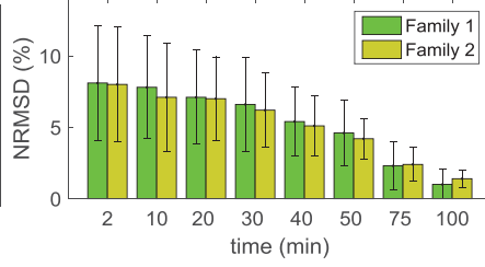
Figure 10: Performance of IAQ forecast algorithm on VOCs prediction at two families.
