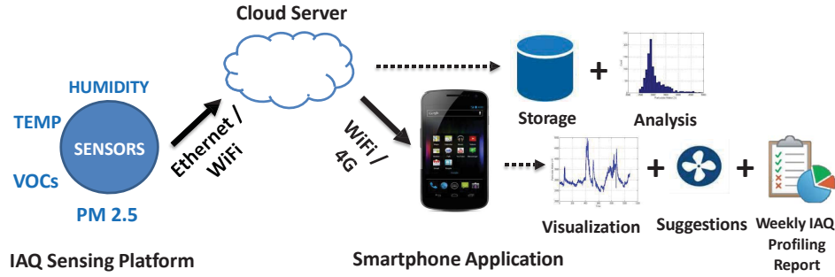
Figure 2: The overview of the system architecture of AirSense.
