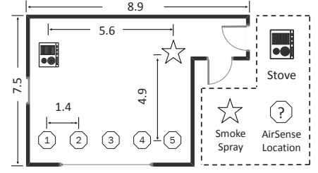
Figure 14: The illustration of the floor plan of the living room and the deployment locations of AirSense (measure unit: meter).
