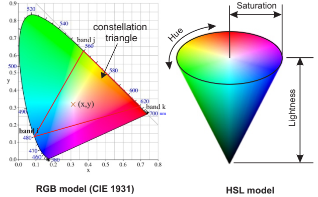
Fig. 3: Illustration of color generation principle (RGB) in Tri-LED and detection principle (HSL) via color filter.
