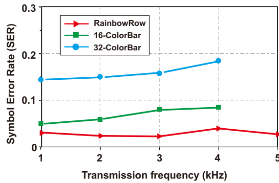
Fig. 12: SER significant reduction compared with state-of-art high-order modulation ColorBar [7].
