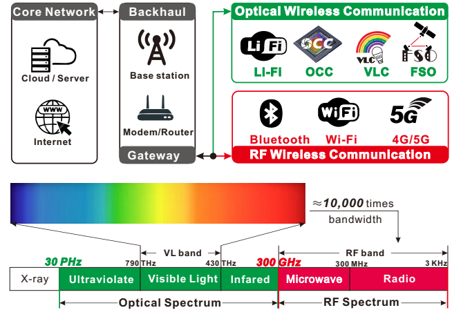
Fig. 1: Optical wireless communication and RF based wireless communication. Optical spectrum has broader bandwidth than RF spectrum.
